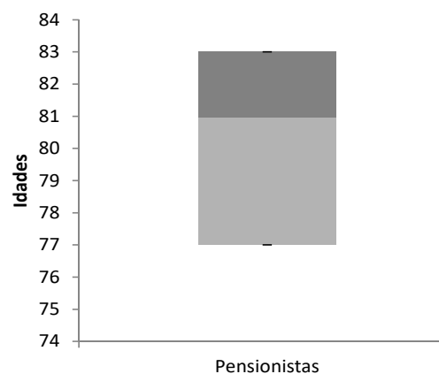
BOXPLOT PENSIONISTAS
